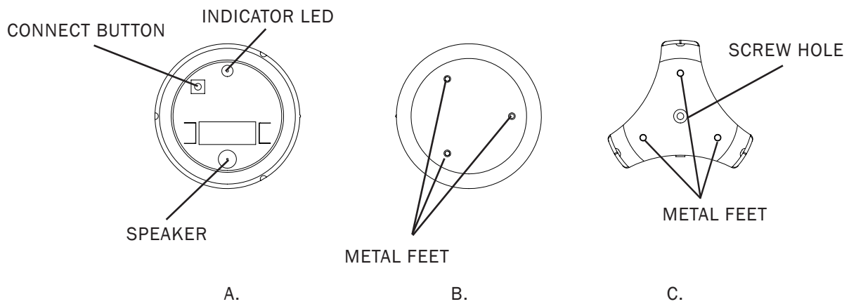
Figure 2 - Showing individual parts A. Inside the Leak Sensor, B. Underneath the Leak Sensor, and C. on the MAIN BODY CRADLE.
